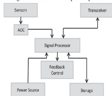
Fig. 2. WBAN Architecture.
